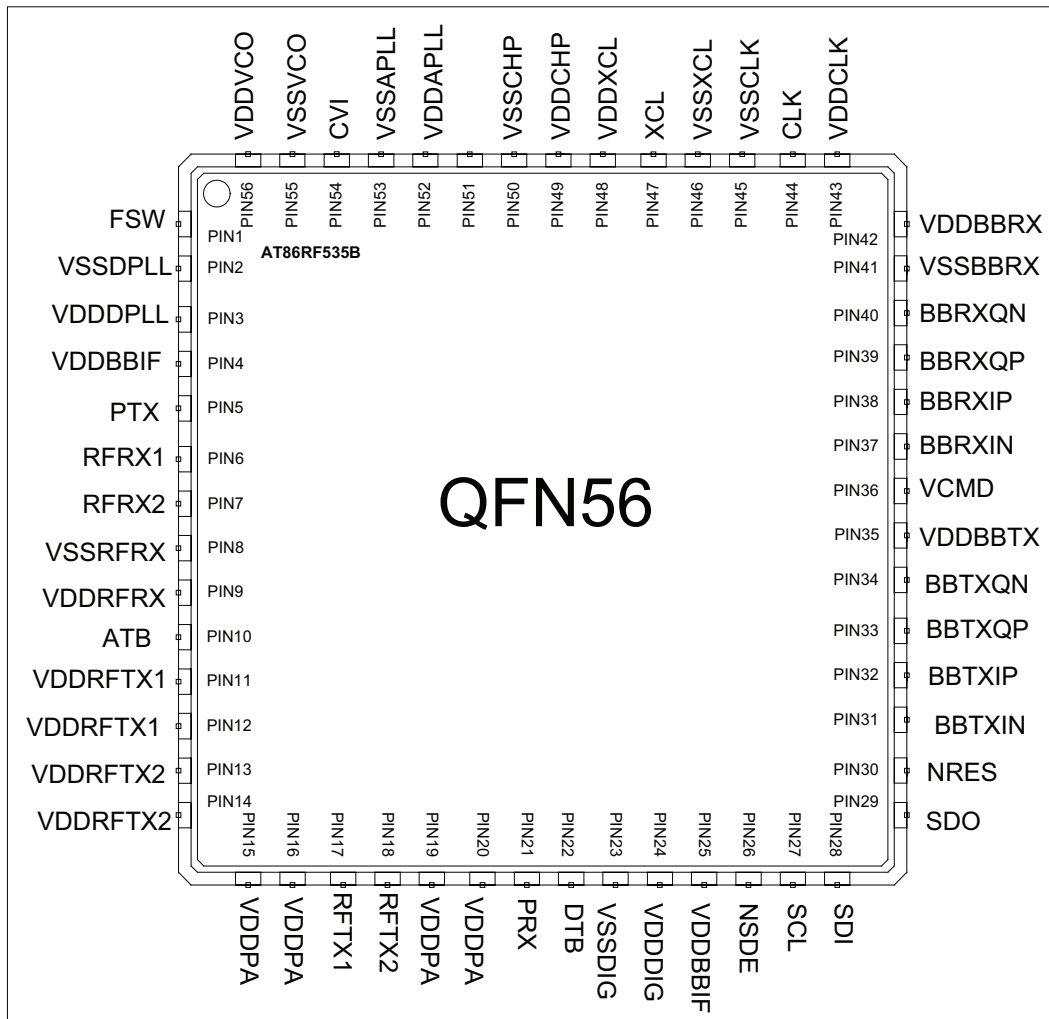
Figure 3. Pin Information
