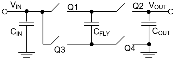
Fig. 11 The circuit of charge pump
