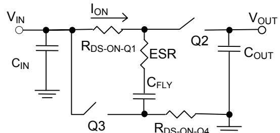
Fig. 12 The on state of charge pump circuit
