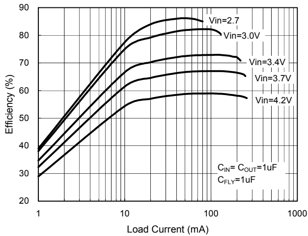
Fig. 7 Efficiency vs. Load Current
