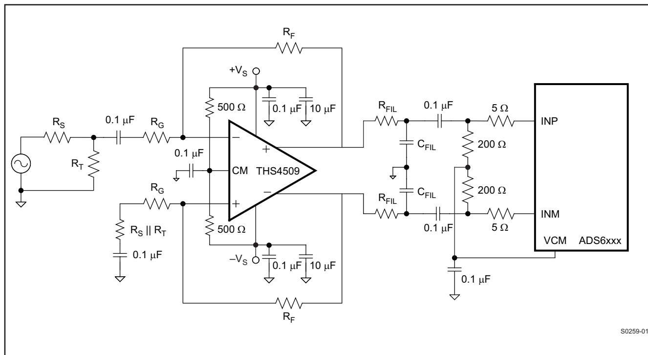
Figure 86. Drive Circuit using THS4509
