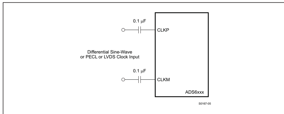
Figure 89. Differential Clock Driving Circuit
