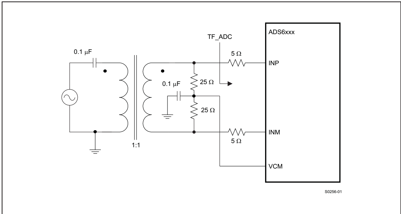
Figure 84. Single Transformer Drive Circuit
