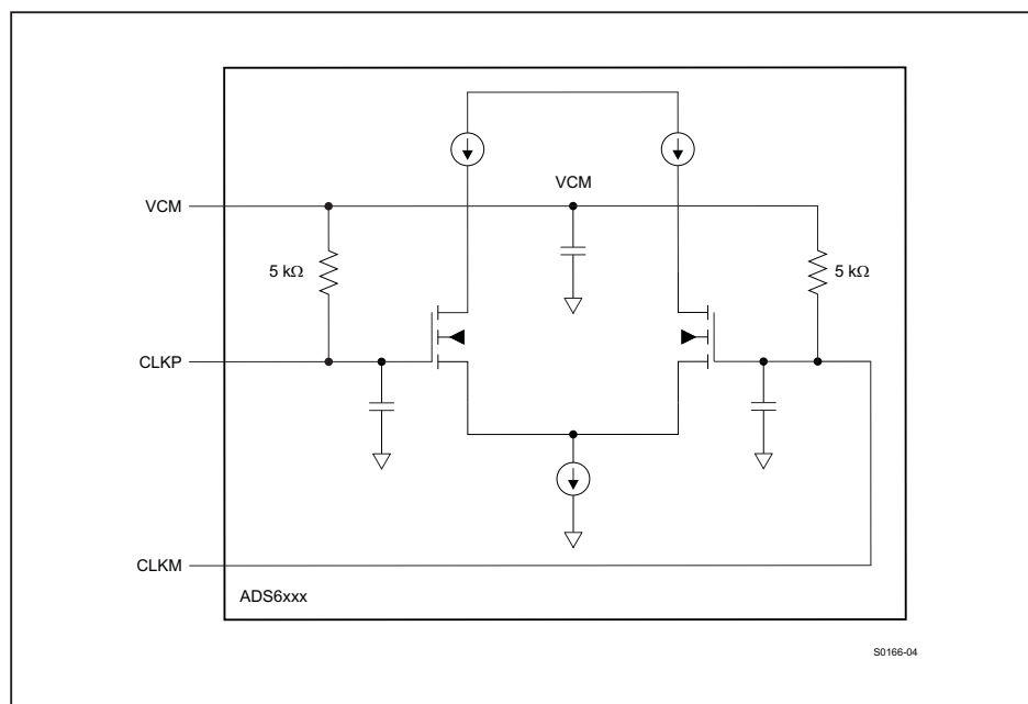
Figure 88. Internal Clock Buffer
