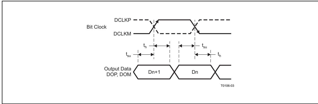
Figure 2. LVDS Timings
