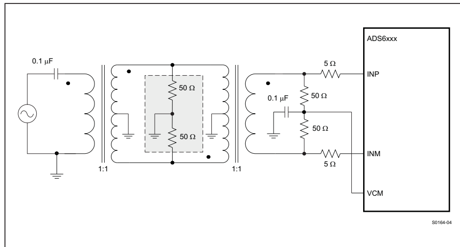
Figure 85. Two Transformer Drive Circuit
