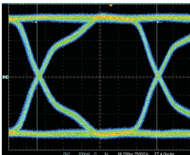
Figure 97. LVDS Data Eye Diagram with 10-pF Load Capacitance (100 \Omega Internal Termination)
