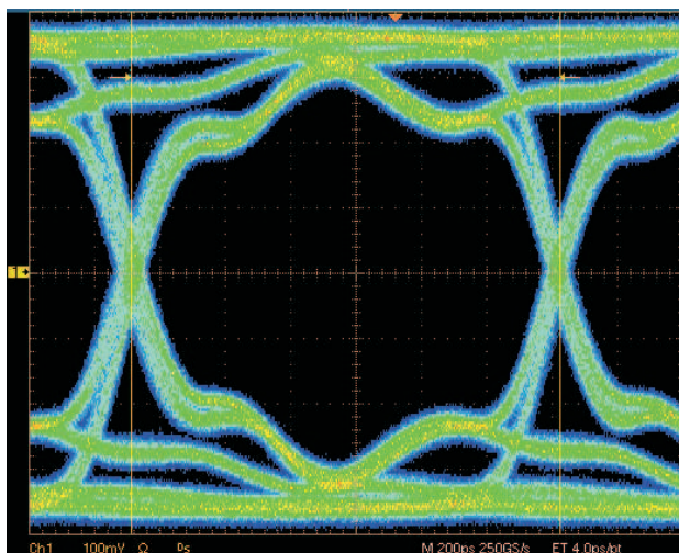
Figure 96. LVDS Data Eye Diagram with 5-pF Load Capacitance (No Internal Termination)
