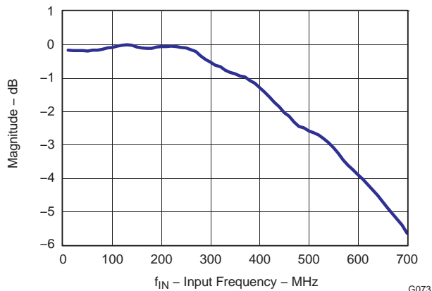
Figure 83. Analog Input Bandwidth (represented by magnitude of TF_ADC, see Figure 84 )
