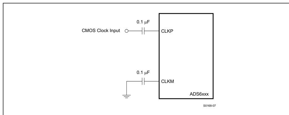
Figure 91. Single-Ended Clock Driving Circuit
