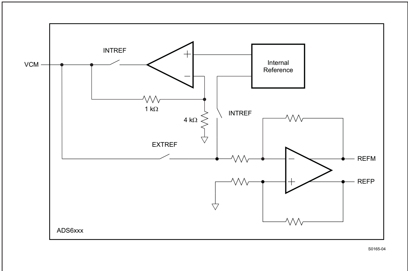
Figure 87. Reference Section
