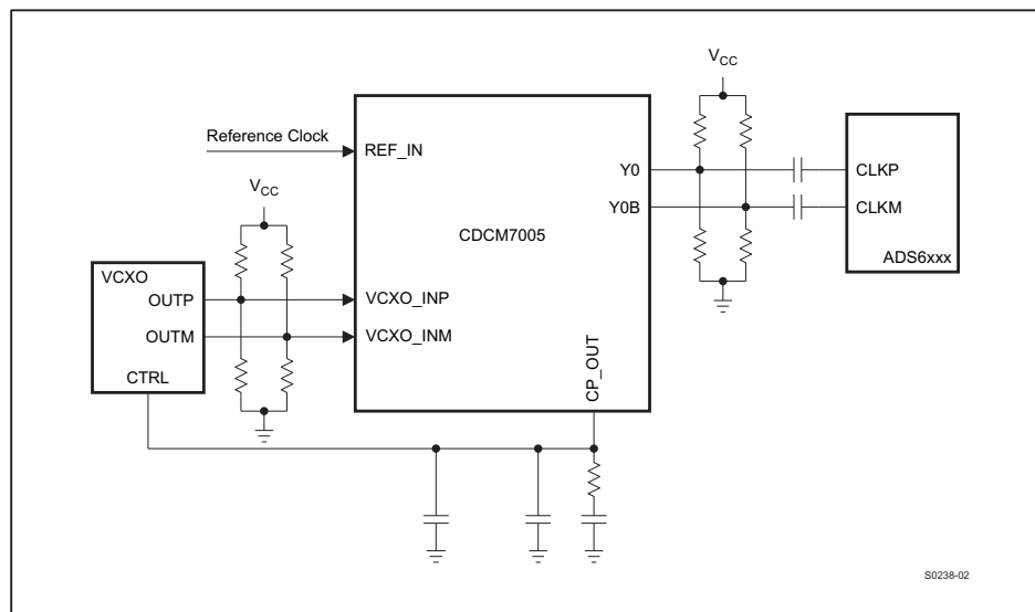
Figure 90. PECL Clock Drive Using CDCM7005
