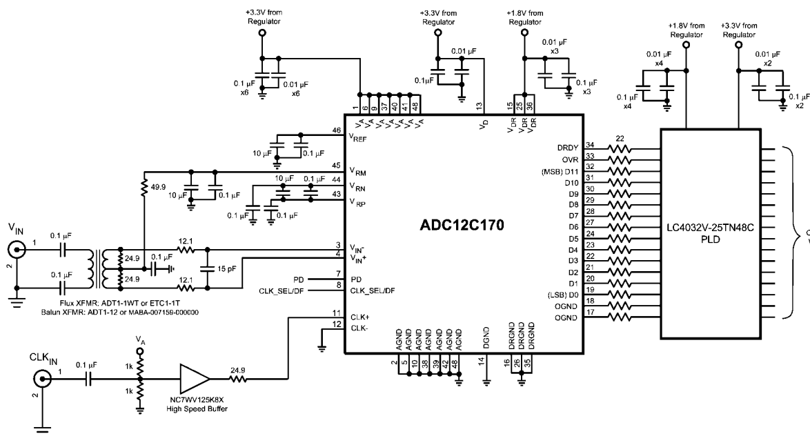
FIGURE 4. Application Circuit using Transformer Drive Circuit (If 14-bit compatibility is not required do not connect pins 17 and 18)
