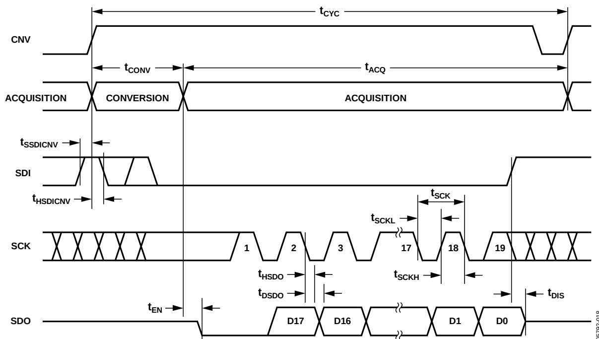
Figure 23. \overline{\text{CS}} Mode 4-Wire with BUSY Indicator Serial Interface Timing
