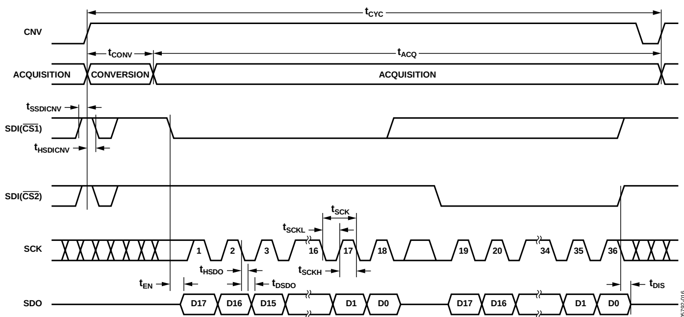
Figure 21. \overline{CS} Mode 4-Wire, No BUSY Indicator Serial Interface Timing
