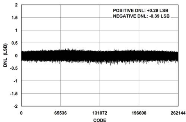
Figure 9. Differential Nonlinearity vs. Code
