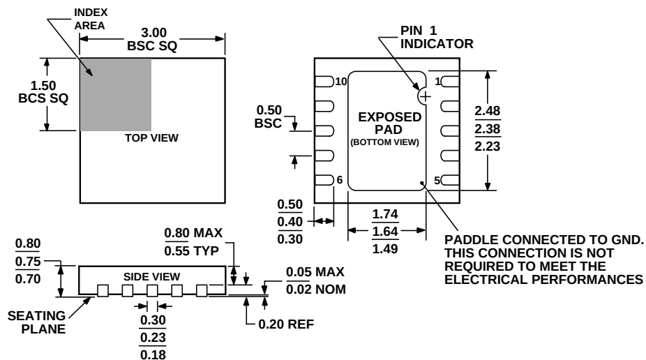
Figure 31. 10-Lead Lead Frame Chip Scale Package [QFN (LFCSP_WD)] 3 mm × 3 mm Body, Very Very Thin, Dual Lead (CP-10-9)
