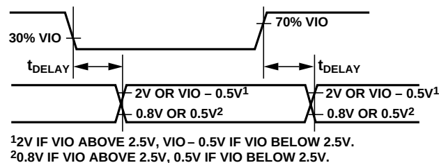
Figure 3. Voltage Levels for Timing
