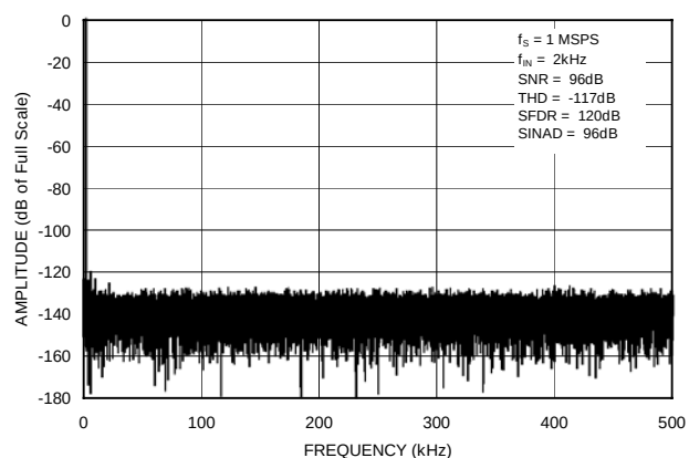
Figure 8. FFT Plot
