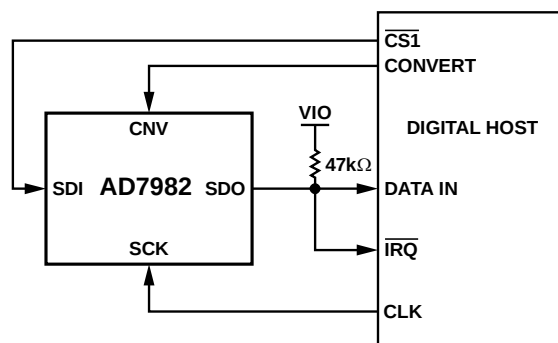
Figure 22. \overline{\text{CS}} Mode 4-Wire with BUSY Indicator Connection Diagram
