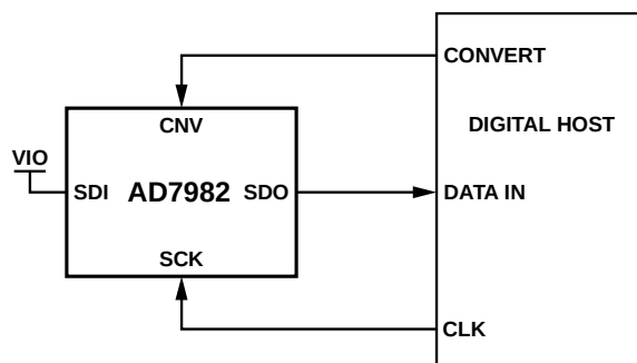
Figure 16. \overline{\text{CS}} Mode 3-Wire, No BUSY Indicator Connection Diagram (SDI High)
