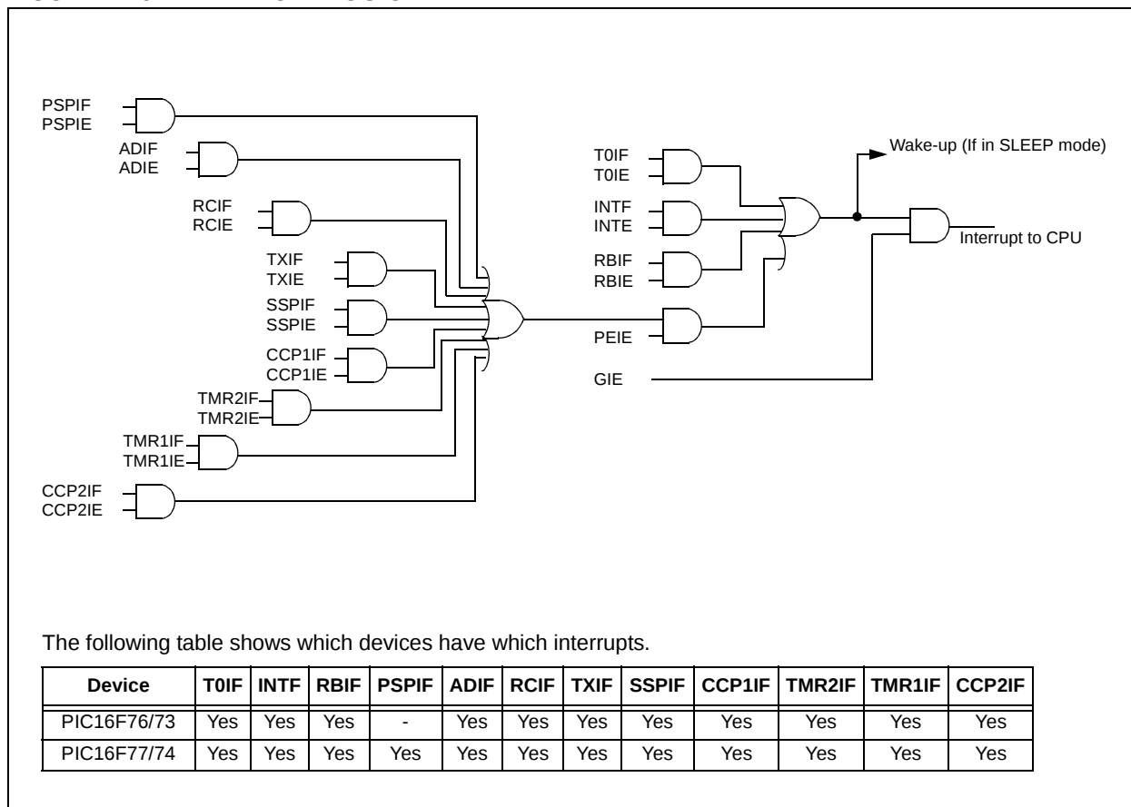
FIGURE 12-9: INTERRUPT LOGIC
