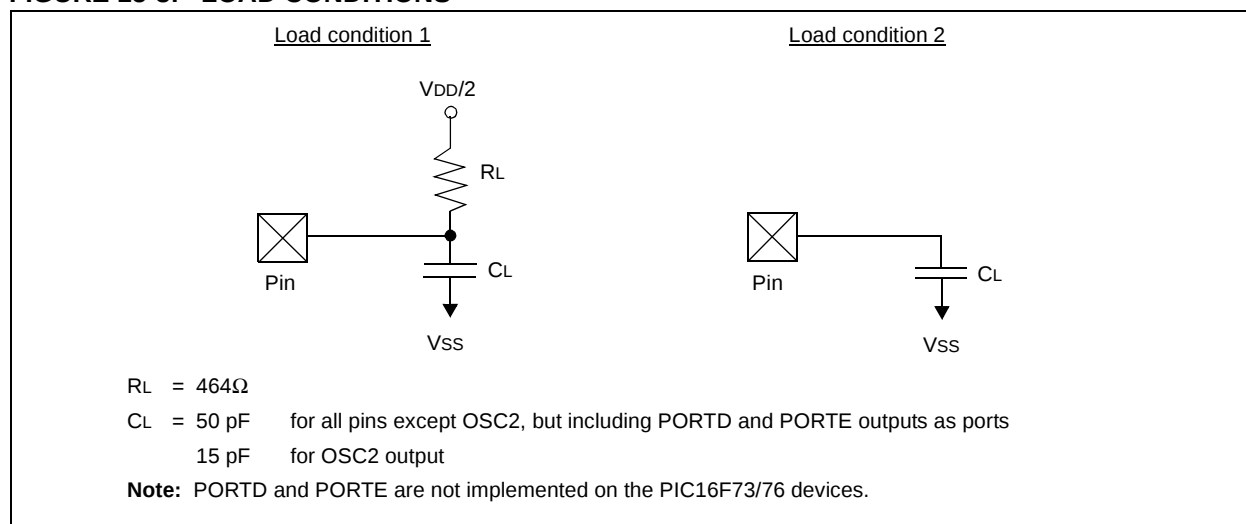
FIGURE 15-3: LOAD CONDITIONS
