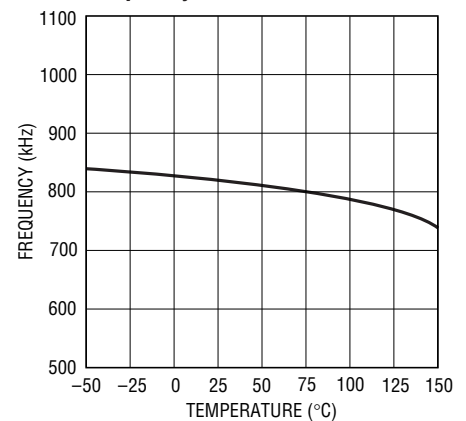
High Voltage Regulator Switch Frequency
