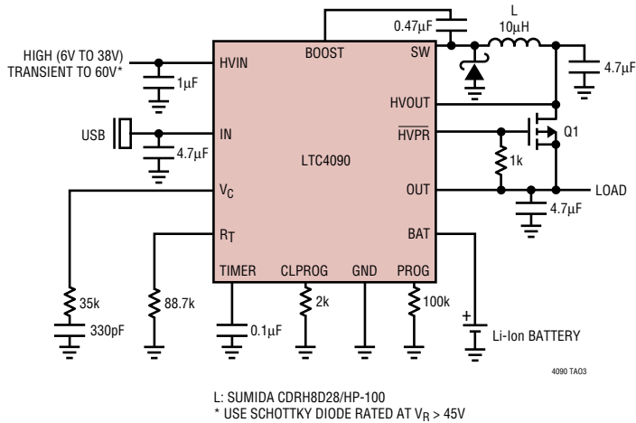
Figure 13. 400kHz Switching Frequency
