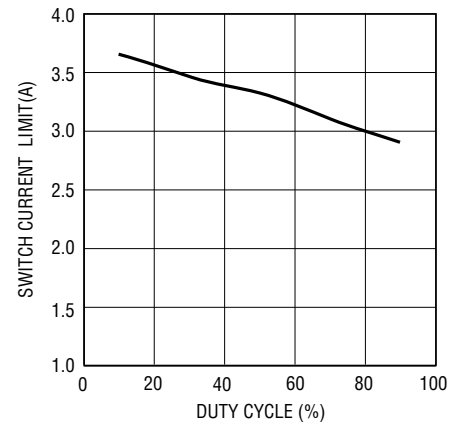
High Voltage Regulator Switch Current Limit
