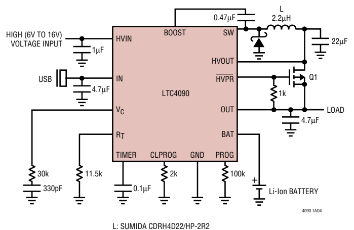
Figure 14. 2MHz Switching Frequency
