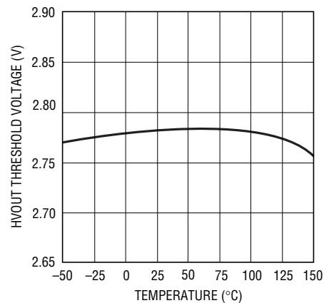
High Voltage Regulator Power Good Threshold
