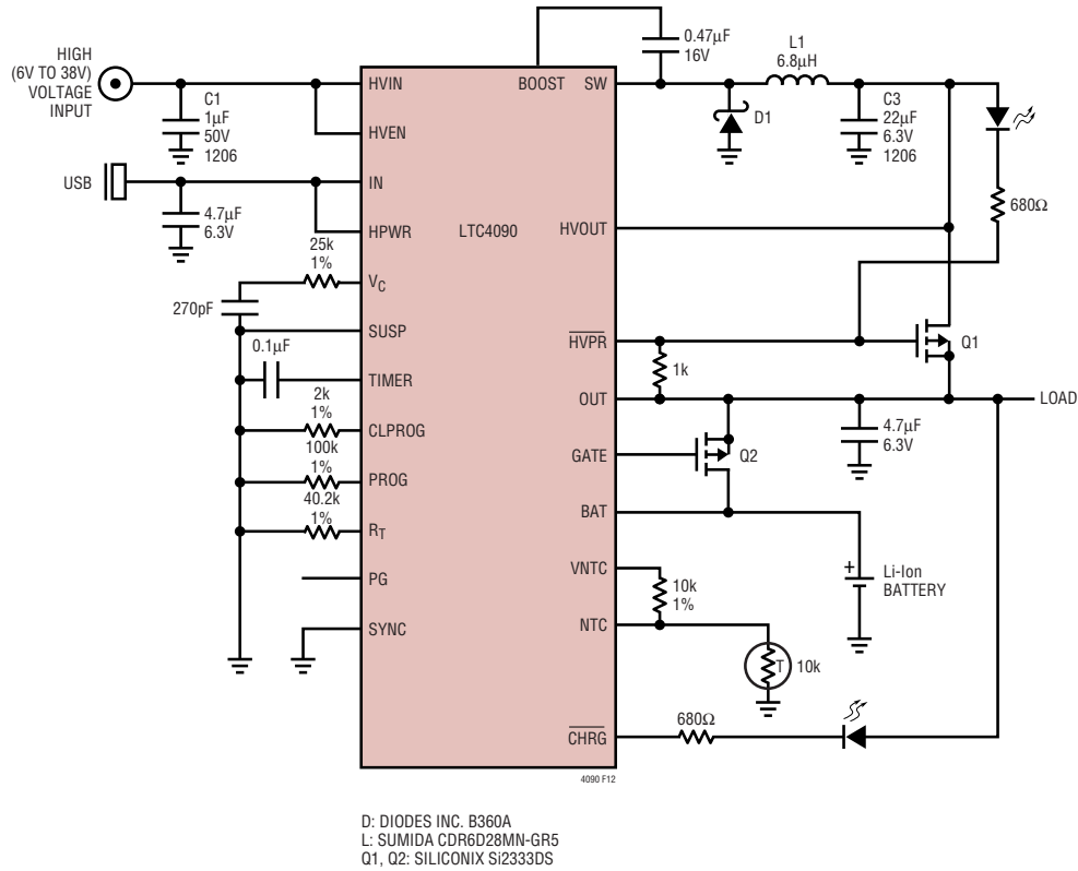
Figure 12. 800kHz Switching Frequency
