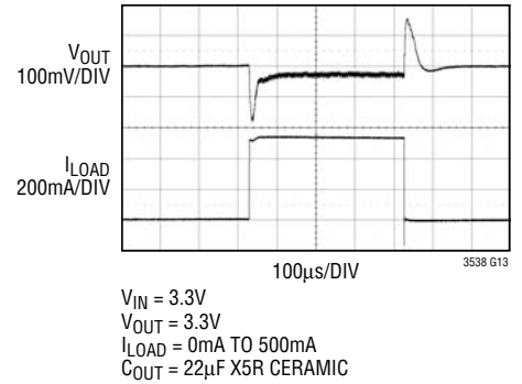
Load Transient in Fixed Frequency Mode
