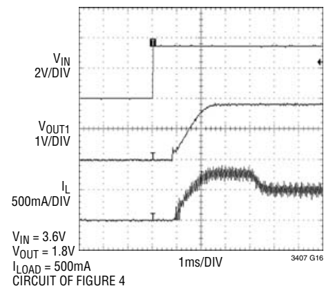
Soft Start
