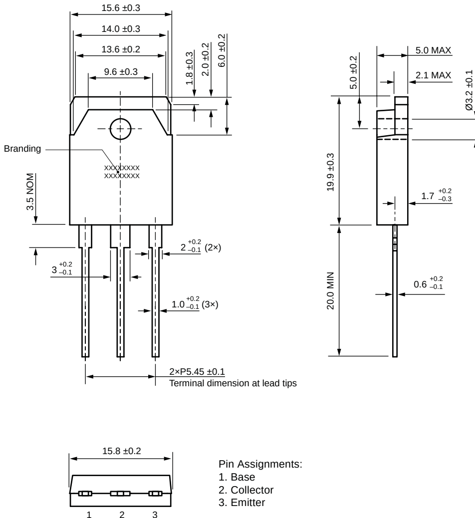
PACKAGE OUTLINE DRAWING, TO-3P
