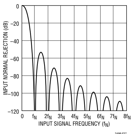
Figure 27. Input Normal Mode Rejection 2x Speed Mode
