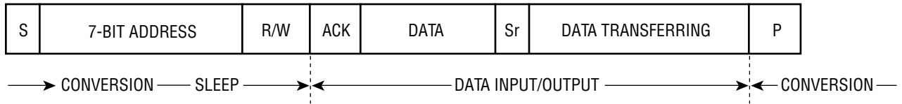
Figure 6. Conversion Sequence
