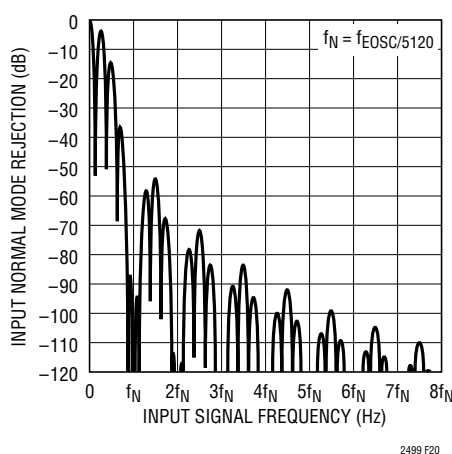
Figure 20. Input Normal Mode Rejection at DC
