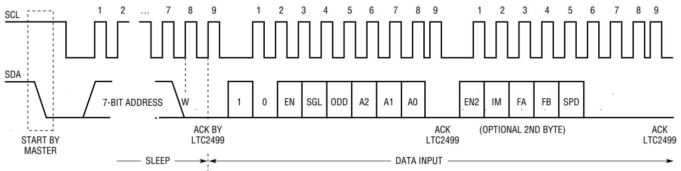
Figure 3b. Timing Diagram for Writing to the LTC2499
