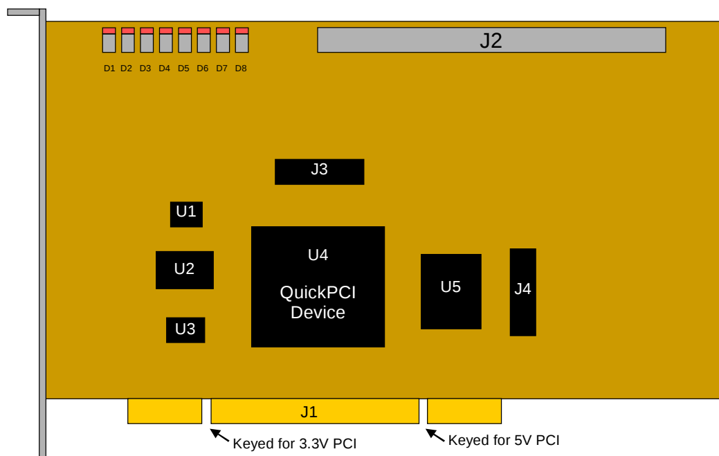
FIGURE 1. QV-PCI32RDK-144 Diagram
