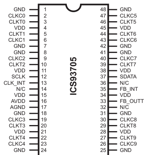
48-Pin SSOP
