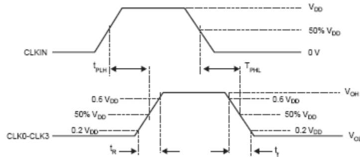
Figure 2. Voltage Thresholds for Propagation Delay ( t_{pd} ) Measurements
