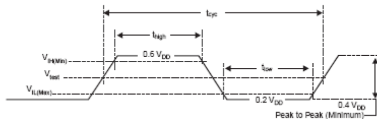
Figure 4. Clock Waveform
