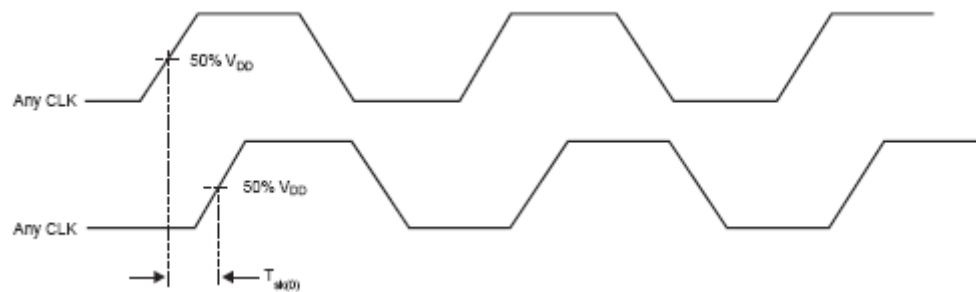
Figure 3. Output Skew
