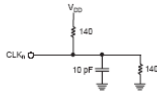
Figure 1. Test Load Circuit
