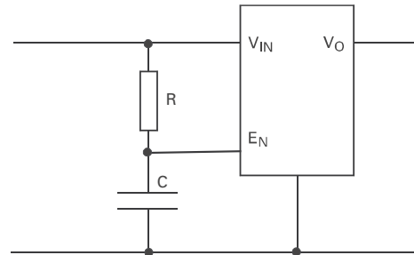
Figure 1 Circuit Connection
