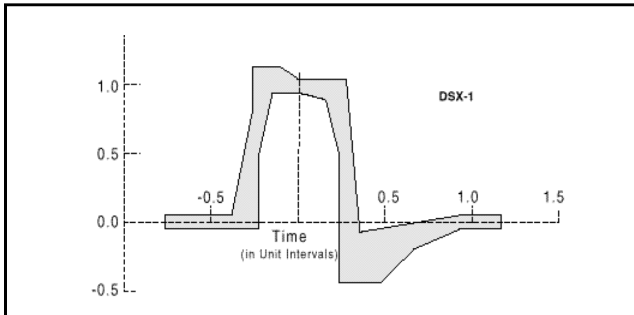
FIGURE 25. DSX-1 PULSE TEMPLATE (NORMALIZED AMPLITUDE)
