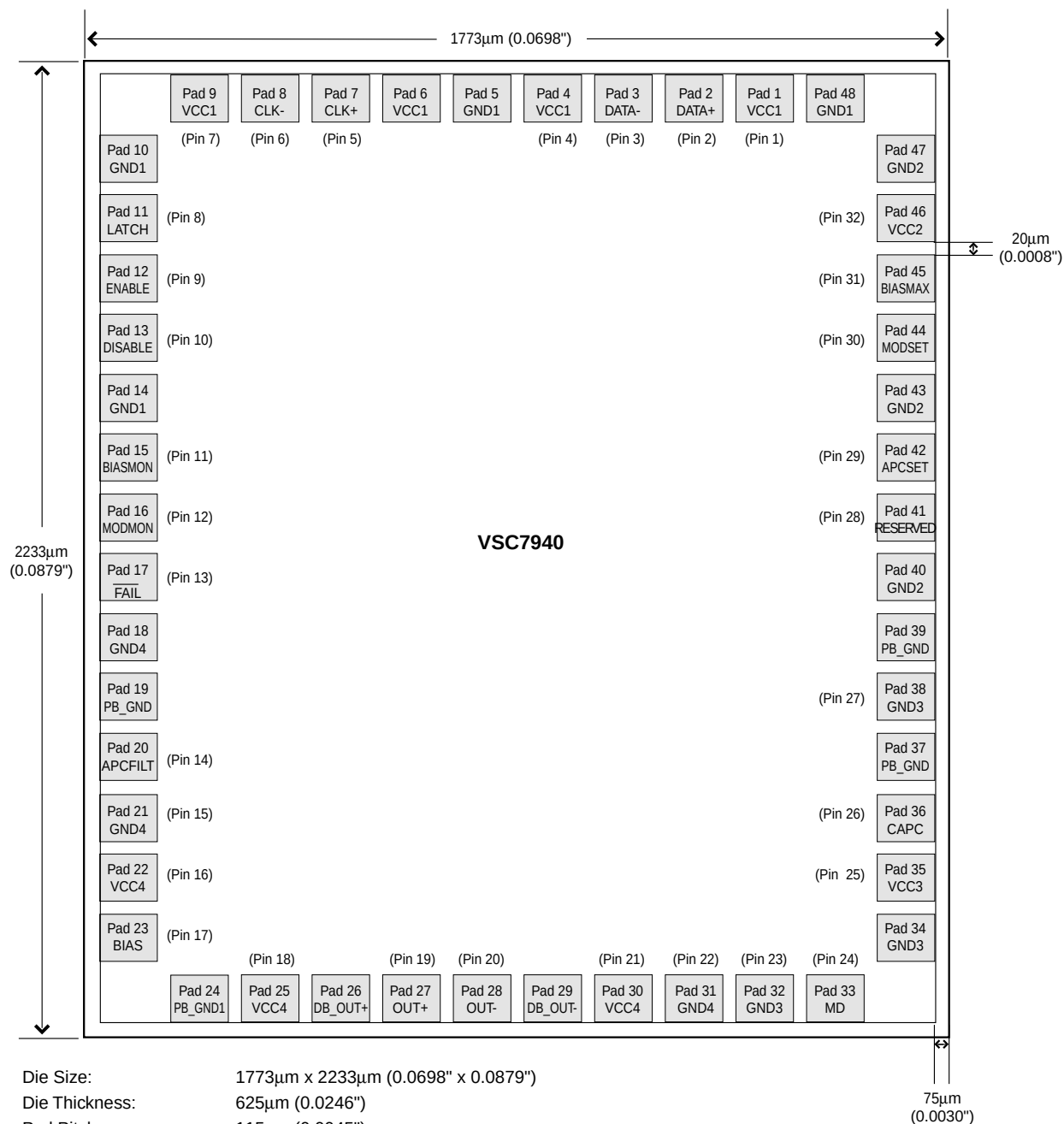
Figure 1: Pad Assignments
