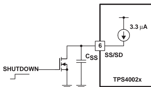
Figure 5. Shutdown Implementation
