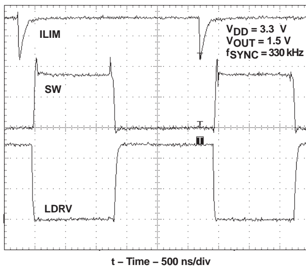
Figure 27. External Synchronization
