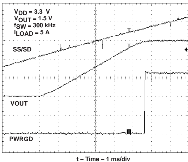
Figure 24. Start-Up Operation With Transient Comparators
