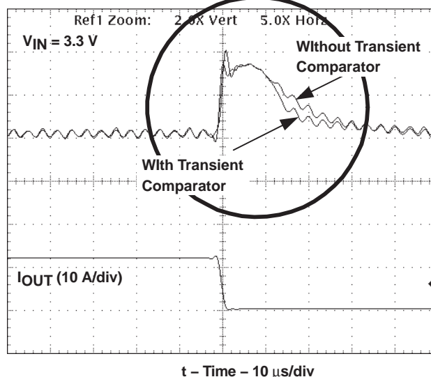
Figure 34. Transient Response Overshoot
