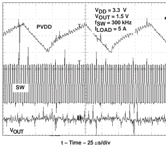
Figure 23. PVDD Hysteresis
