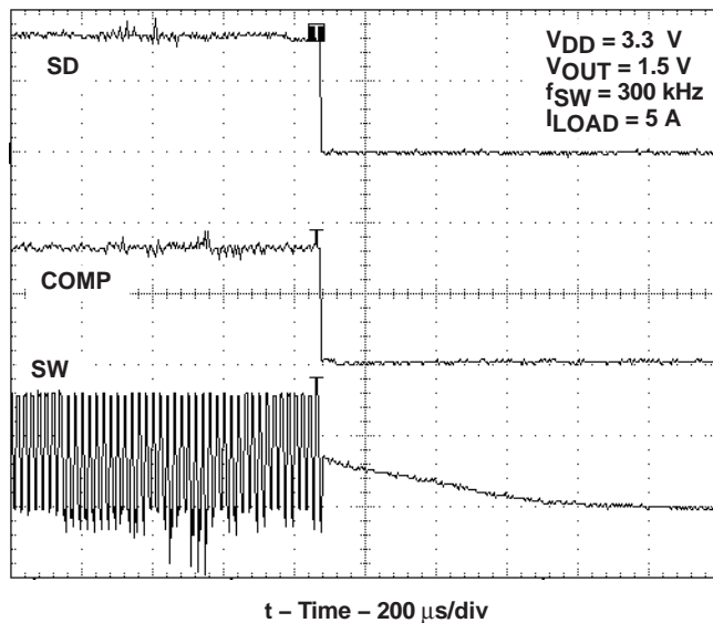
Figure 25. COMP Shutdown Operation
