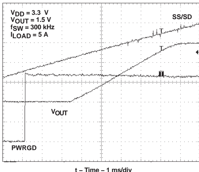
Figure 22. Start-Up Operation Without Transient Comparators
