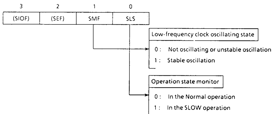
Figure 3-6. Command register and Status register
