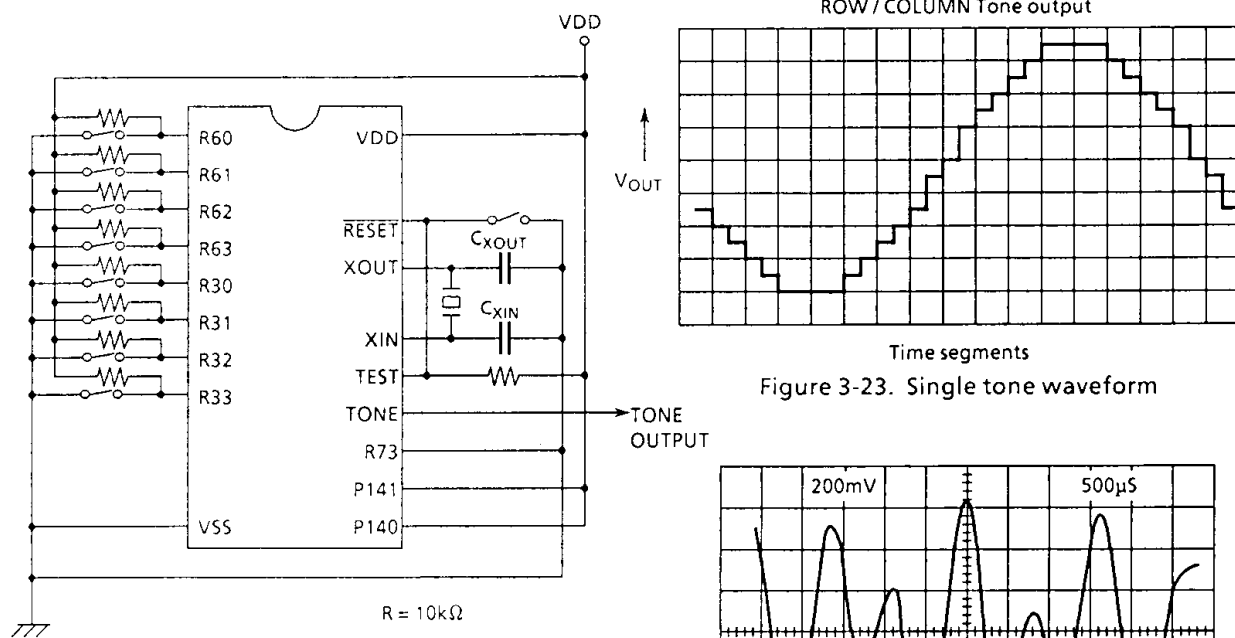
Figure 3-22. Tone test circuit
