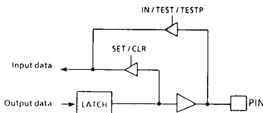
Figure 3-2. Port R3
