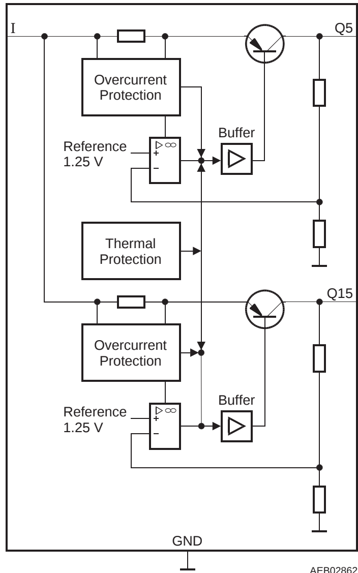
Figure 2 Block Diagram
