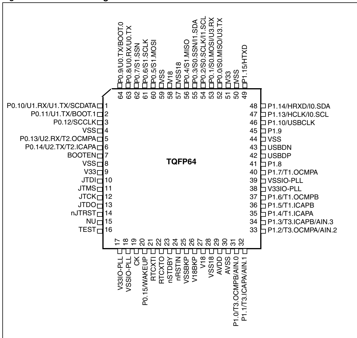
Figure 4. STR711F Package Pinout
