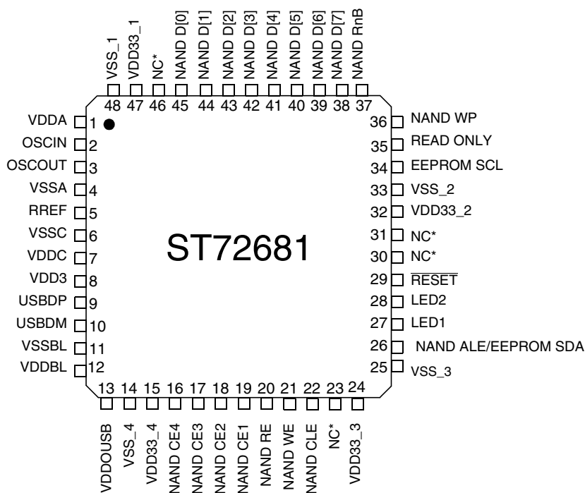
Figure 2. 48-Pin TQFP Package Pinout
