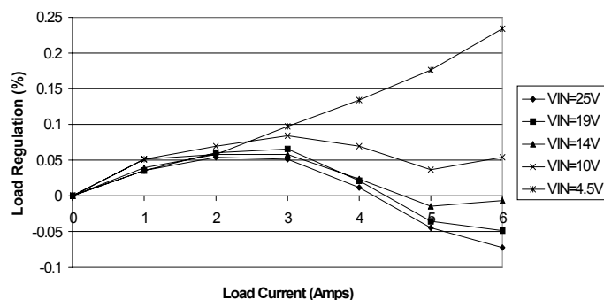
SC1485 Load Regulation at V_{out} = 3.3V
