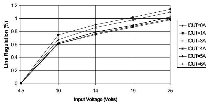
SC1485 Line Regulation at V_{out} = 3.3V
