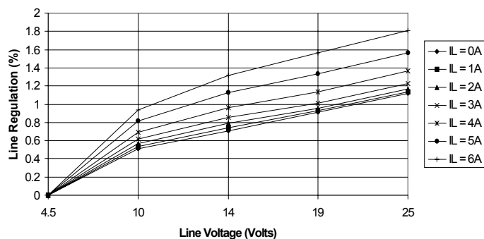
SC1485EVB Line Regulation at V_{out} = 1.8V
