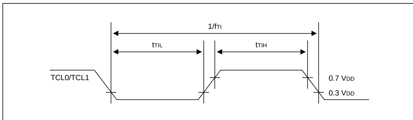
Figure 15-7. TCL0/TCL1 Timing
