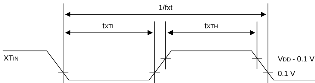
Figure 15-6. Clock Timing Measurement at XT_{IN}
