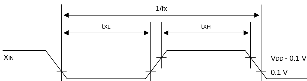
Figure 15-5. Clock Timing Measurement at X_{IN}
