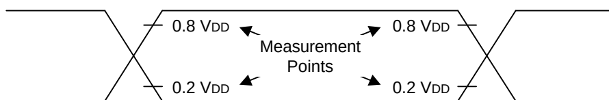
Figure 15-4. A.C. Timing Measurement Points (Except for X_{IN} and XT_{IN} )
