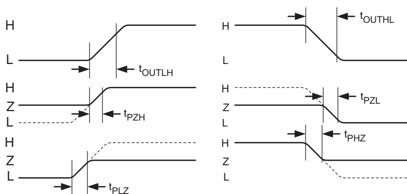
Figure 15: Eclipse Output Register Cell Timing
