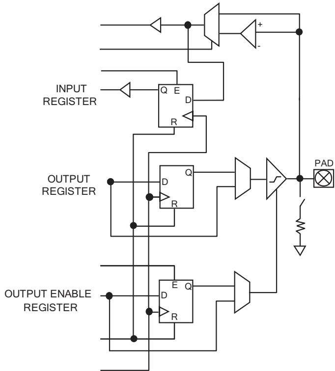
Figure 11: Eclipse Cell I/O
