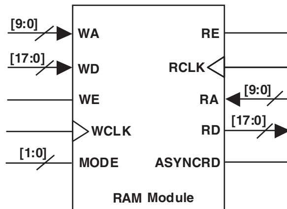
Figure 12: RAM Module
