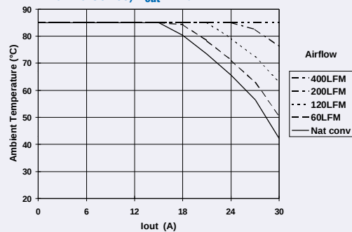
PT8120 Series, V_{out} = 1.5V
