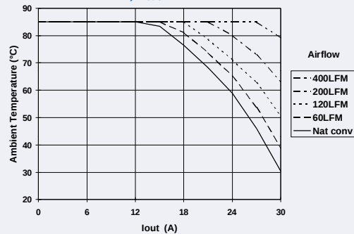
PT8120 Series, V_{out} = 3.3V
