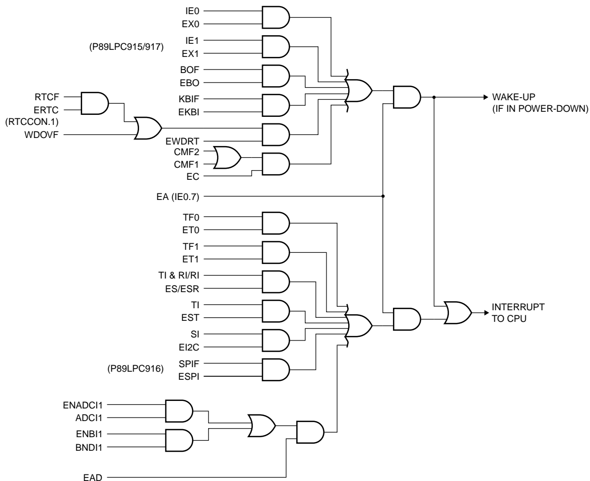
Fig 12. Interrupt sources, interrupt enables, and power-down wake-up sources.
