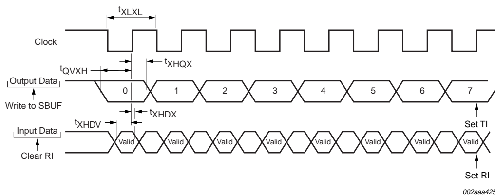
Fig 26. Shift register mode timing.
