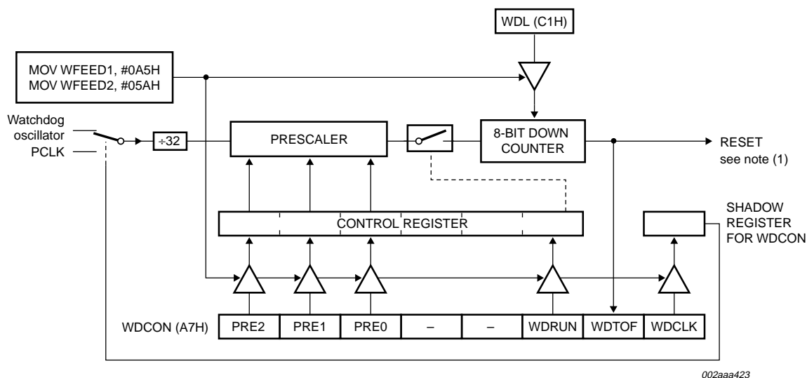
Fig 21. Watchdog timer in Watchdog mode (WDTE = 1).
