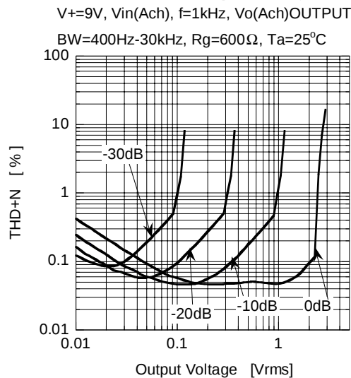
THD+N vs Output Voltage
