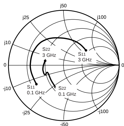
Coordinates in Ohms Frequency in GHz V_{CE} = 12\text{ V} , I_C = 100\text{ mA}
