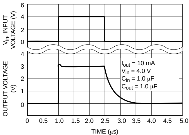
Figure 11. Turn-on Response
