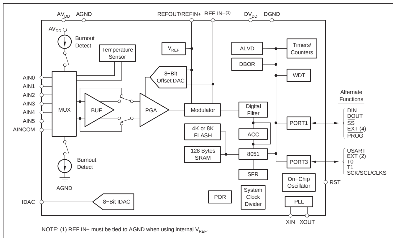
Figure 3. Block Diagram
