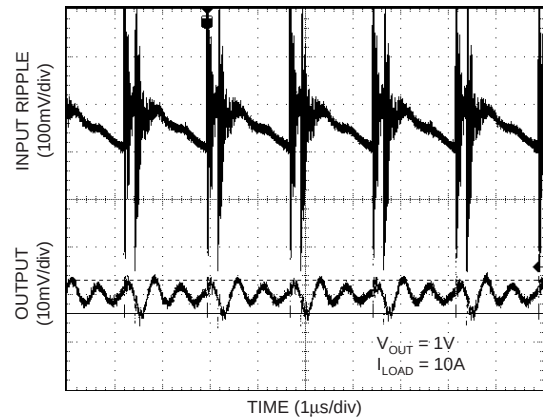
Figure 11. Ripple Reduction
