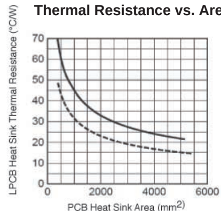
Figure 8. PC Board Heat Sink
