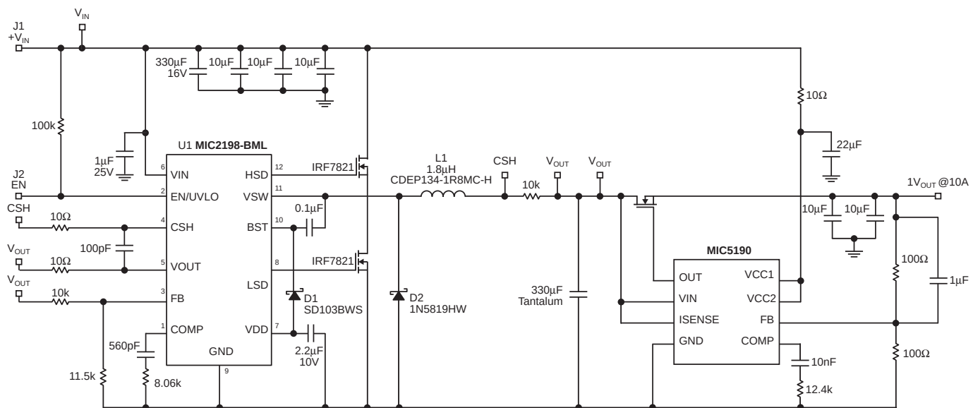
Figure 9. Post Regulator
