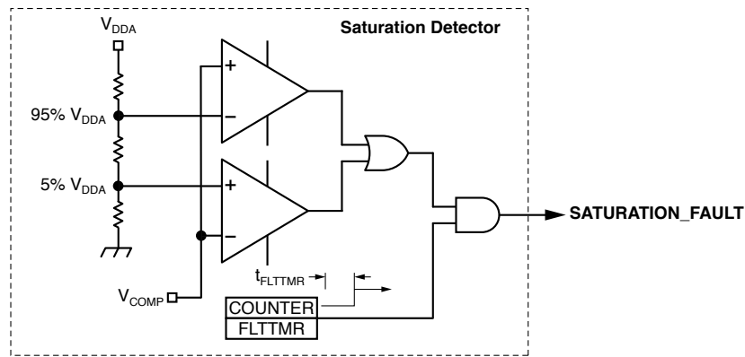
Figure 9. Saturation Detector
