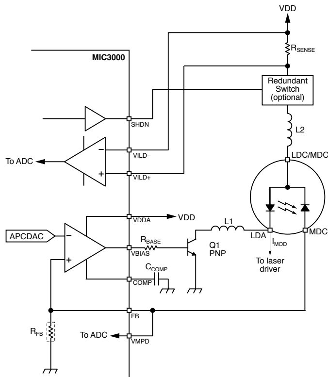
Figure 26. Example APC Circuit for Common Anode TOSA
