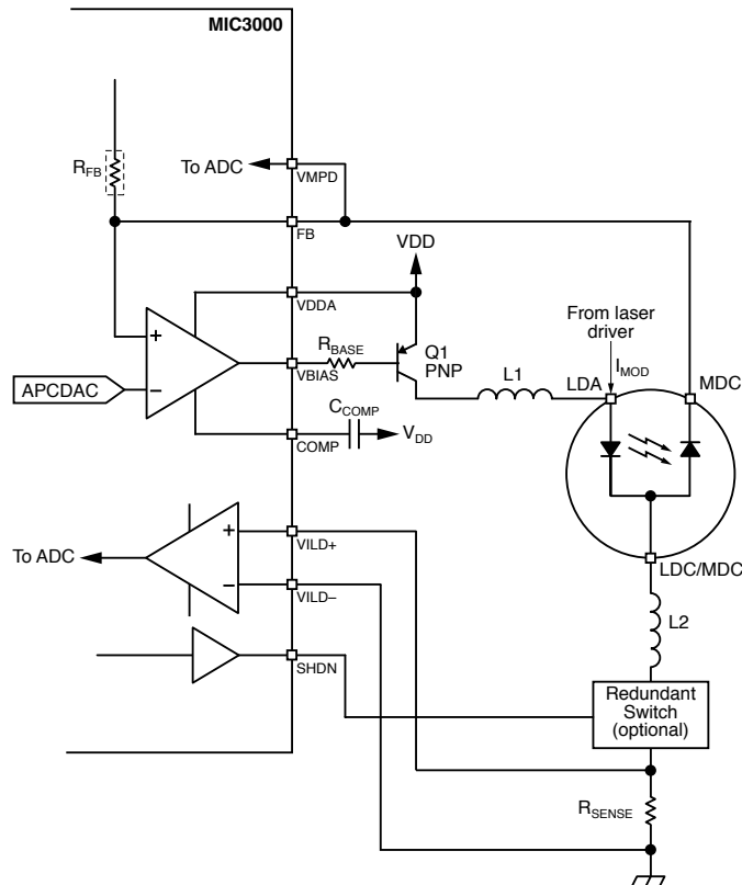
Figure 25. Example APC Circuit for Common-Cathode TOSA
