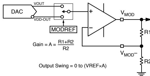
Figure 6. V MOD Configured as Voltage Output with Gain
