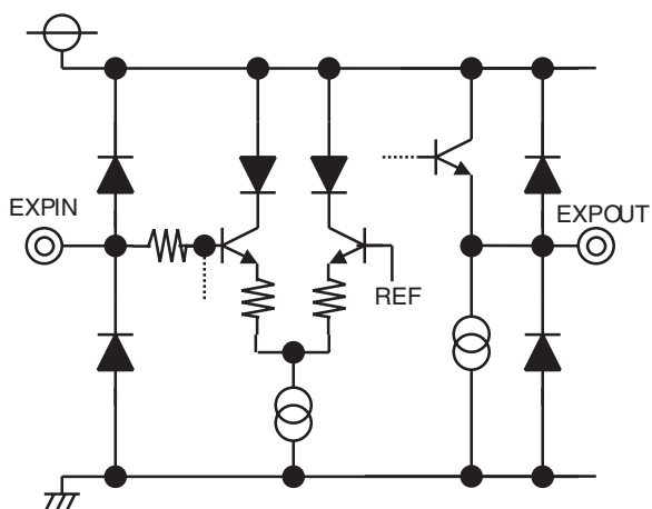
17 EXPIN, EXPOUT
