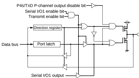
(5) Port P45
