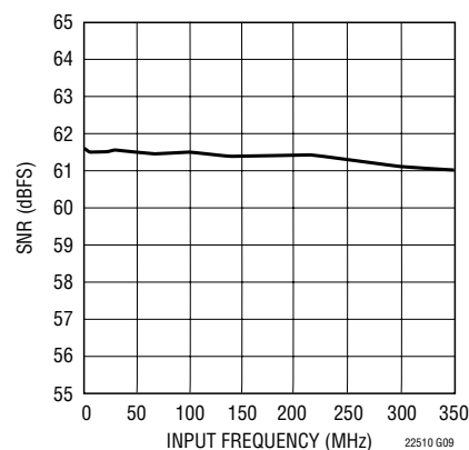
LTC2251: SNR vs Input Frequency, -1dB, 2V Range, 125Mpsps
