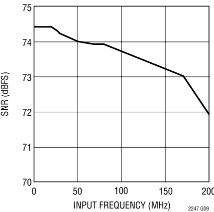
LTC2247: SNR vs Input Frequency, -1\text{dB} , 2\text{V} Range, 40\text{Mpsps}
