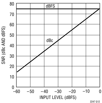
LTC2247: SNR vs Input Level, f_{IN} = 5\text{MHz} , 2\text{V} Range, 40\text{Mpsps}
