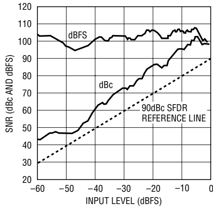
LTC2247: SFDR vs Input Level, f_{IN} = 5\text{MHz} , 2V Range, 40Msps
