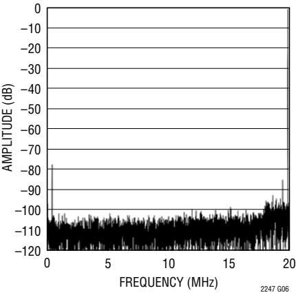
LTC2247: 8192 Point FFT, f_{IN} = 140\text{MHz} , -1\text{dB} , 2\text{V} Range, 40\text{Mpsps}
