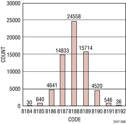
LTC2247: Grounded Input Histogram, 40\text{Mpsps}
