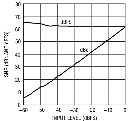
LTC2237: SNR vs Input Level, f_{IN} = 5\text{MHz} , 2V Range, 40Msps
