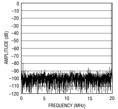
LTC2237: 8192 Point FFT, f_{IN} = 140\text{MHz} , -1\text{dB} , 2V Range, 40Msps
