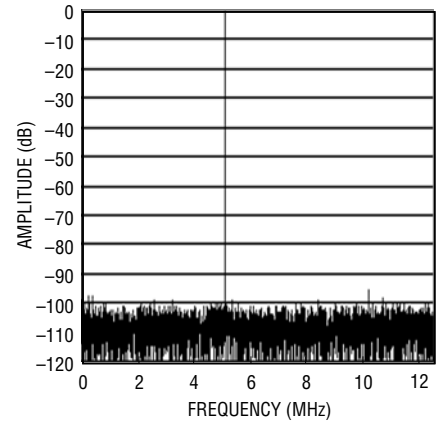
LTC2226: 8192 Point FFT, f_{IN} = 5\text{MHz} , -1dB, 2V Range, 25Msps
