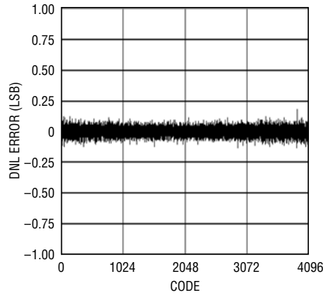
LTC2226: Typical DNL, 2V Range, 25Msps
