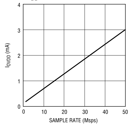
LTC2227: I_{VDD} vs Sample Rate, 5MHz Sine Wave Input, -1dB, OV_{DD} = 1.8\text{V}
