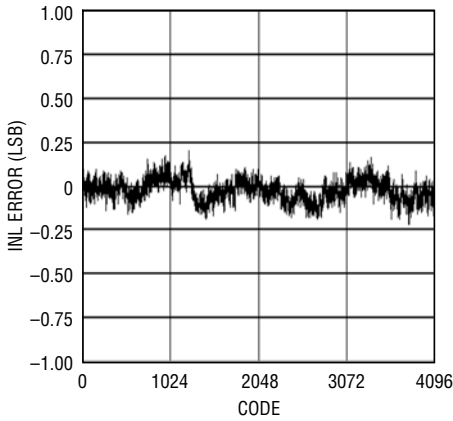
LTC2226: Typical INL, 2V Range, 25Msps
