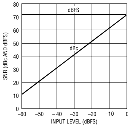
LTC2228: SNR vs Input Level, f_{IN} = 30\text{MHz} , 2V Range, 65Mpsps
