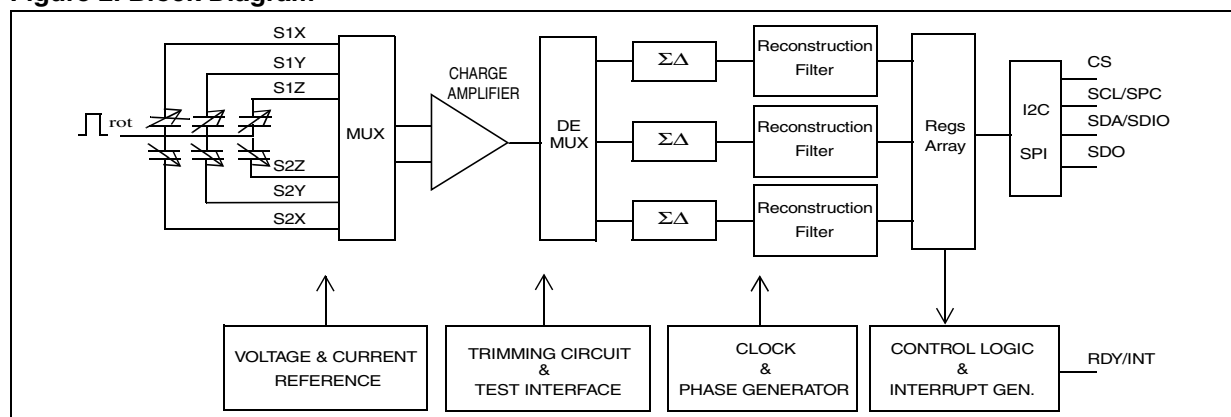
Figure 2. Block Diagram
