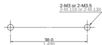
Panel cutout
