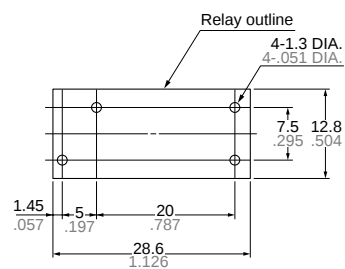
PC board pattern (Copper-side view)
