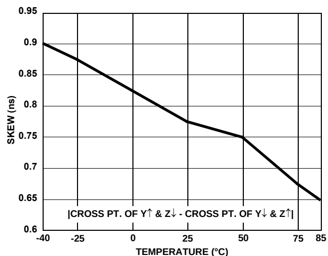
FIGURE 16. DRIVER DIFFERENTIAL SKEW vs TEMPERATURE (ISL83076E, ISL83078E)
