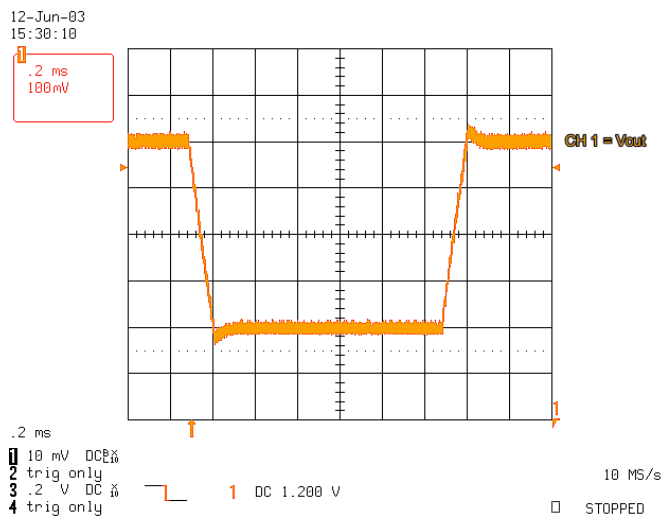
FIGURE 6. VID CHANGES FROM 1.60V TO 1.20V
