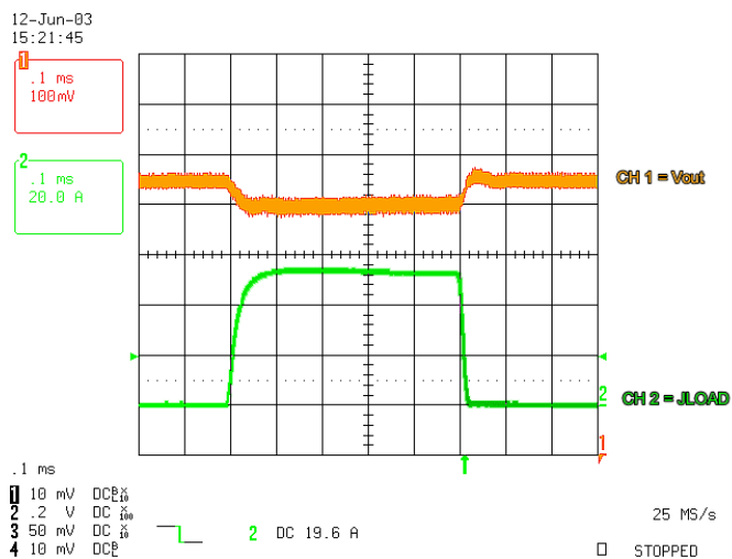
FIGURE 4. TRANSIENT WAVEFORM FROM 0A TO 52A
