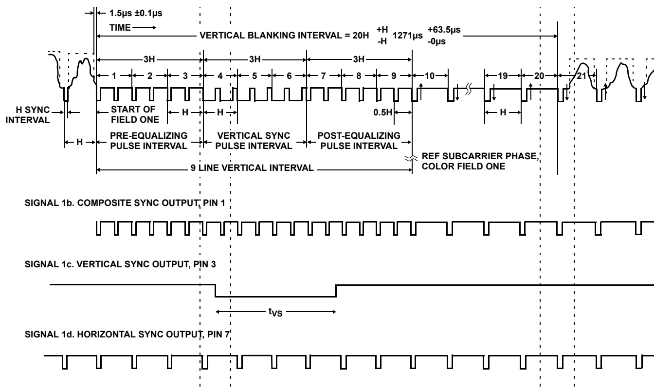
SIGNAL 1a. COMPOSITE VIDEO INPUT, FIELD ONE
