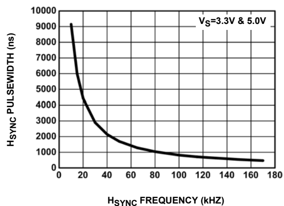
FIGURE 2. H_{SYNC} PULSEWIDTH vs H_{SYNC} FREQUENCY ( R_{SET} = OPEN )
