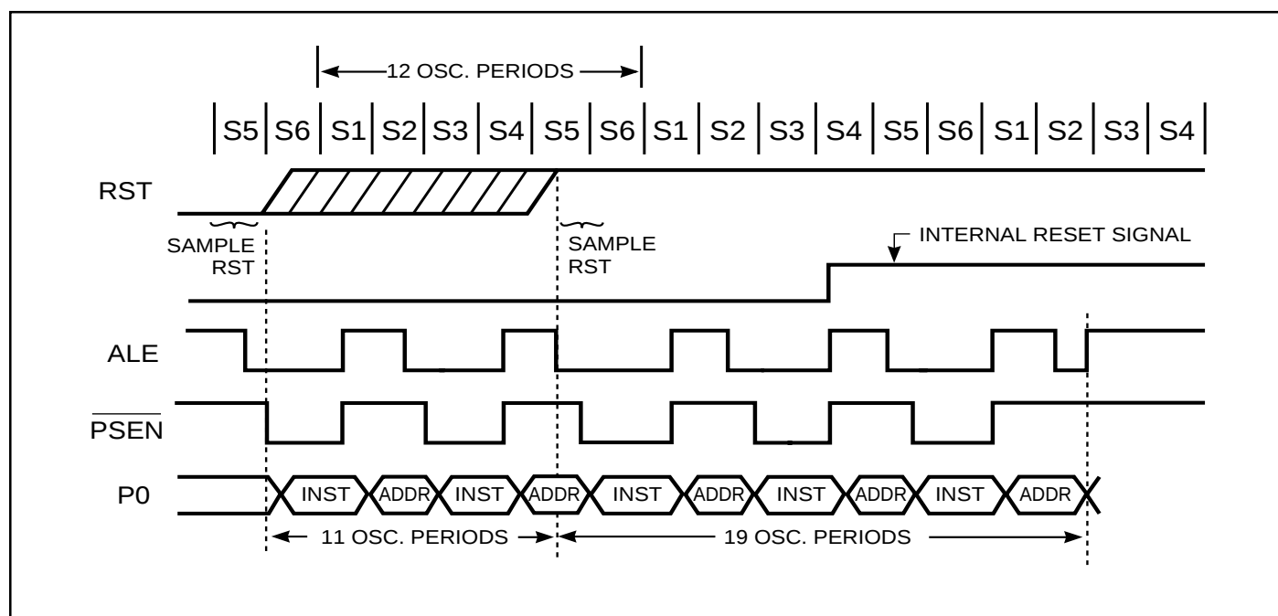
Figure 19. Reset Timing
