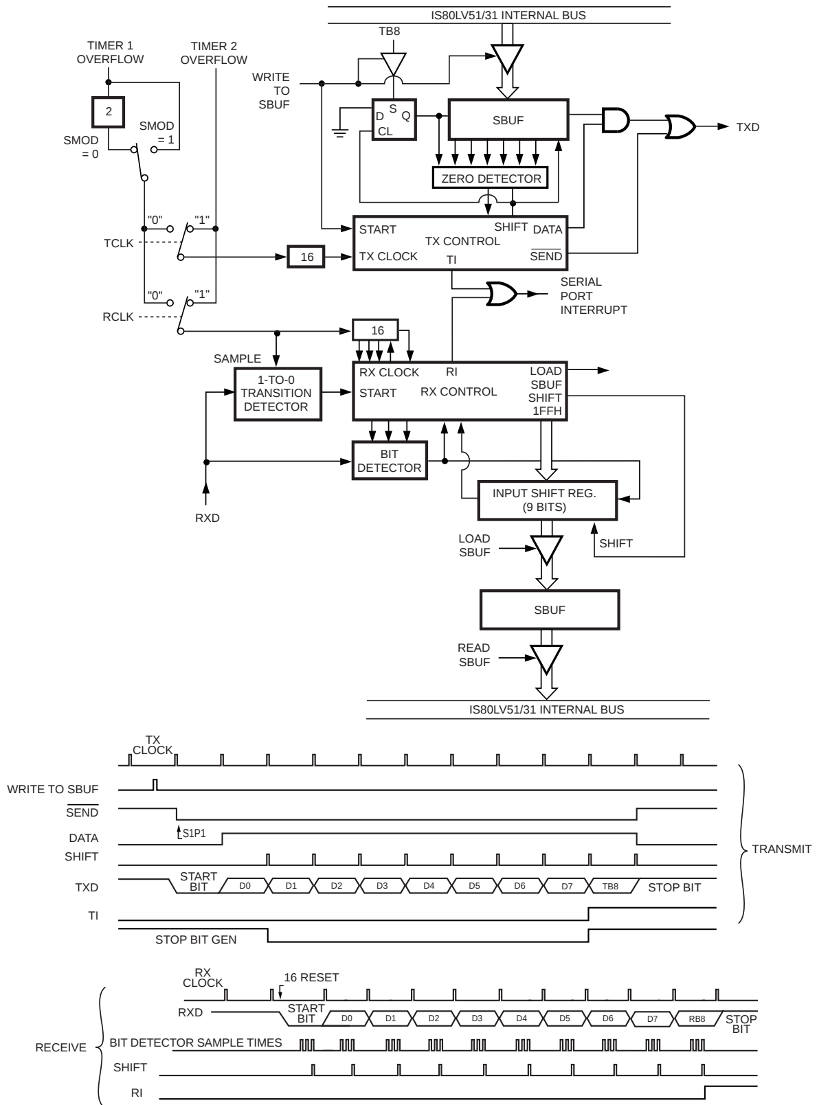
Figure 15. Serial Port Mode 3
