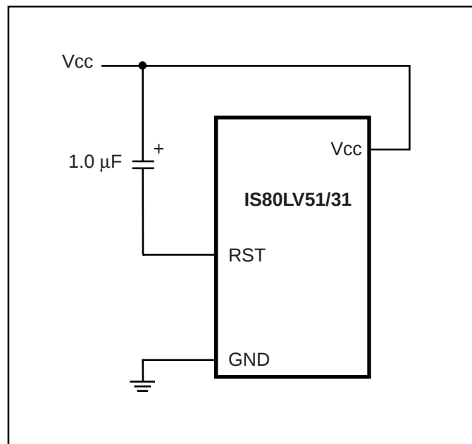
Figure 18. Power-On Reset Circuit
