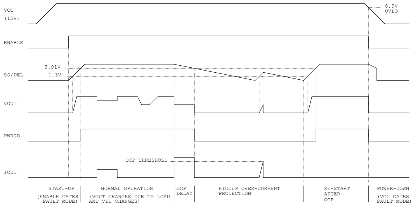
Figure 11 – Operating Waveforms
