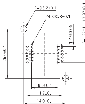
SOP IC51-0242-793 (24 Pins)
