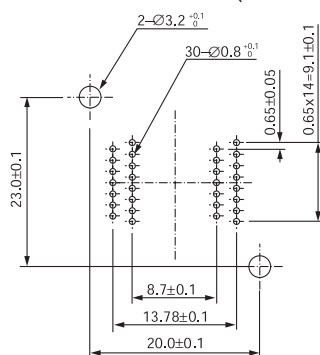
SSOP IC51-0302-914 (30 Pins)
