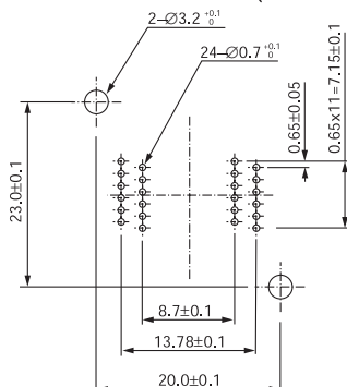
SSOP IC51-0242-761 (24 Pins)
