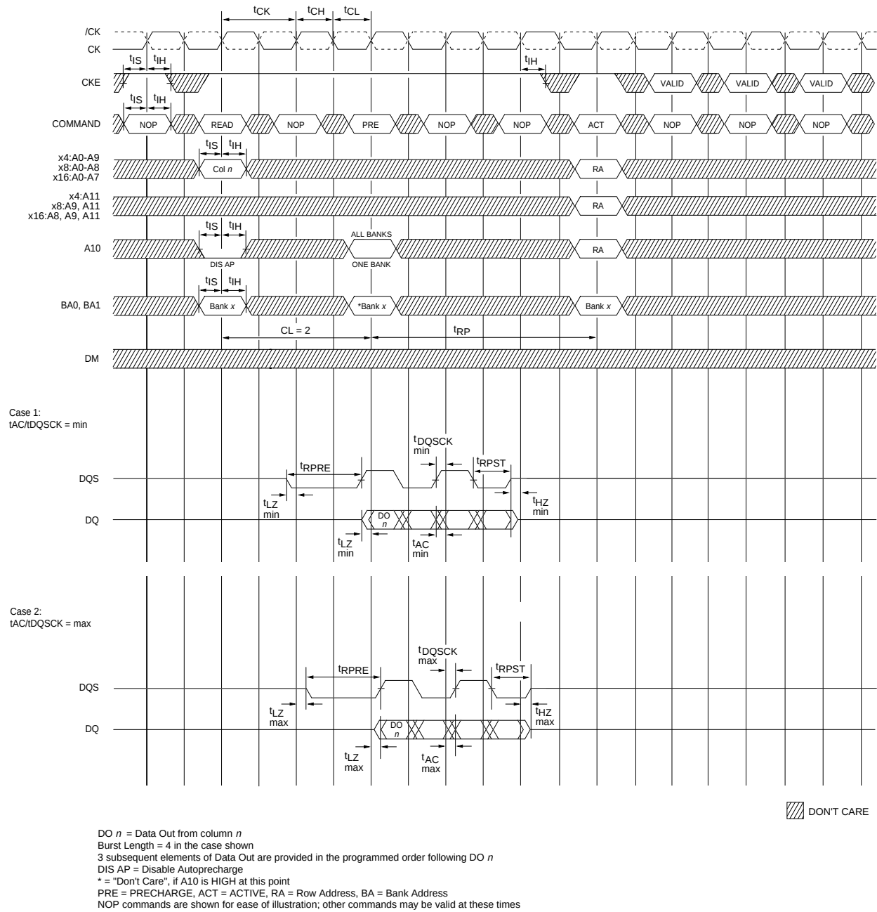
Figure 43 - READ - WITH AUTO PRECHARGE
