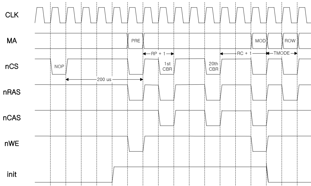
Figure 2.8 Initialization timing
